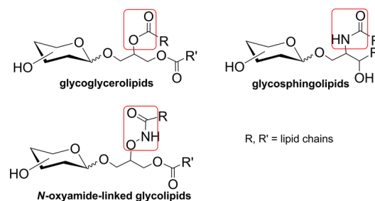
Figure 1. Structure of GGLs, GSLs, and N -oxyamide-linked glycolipids.
